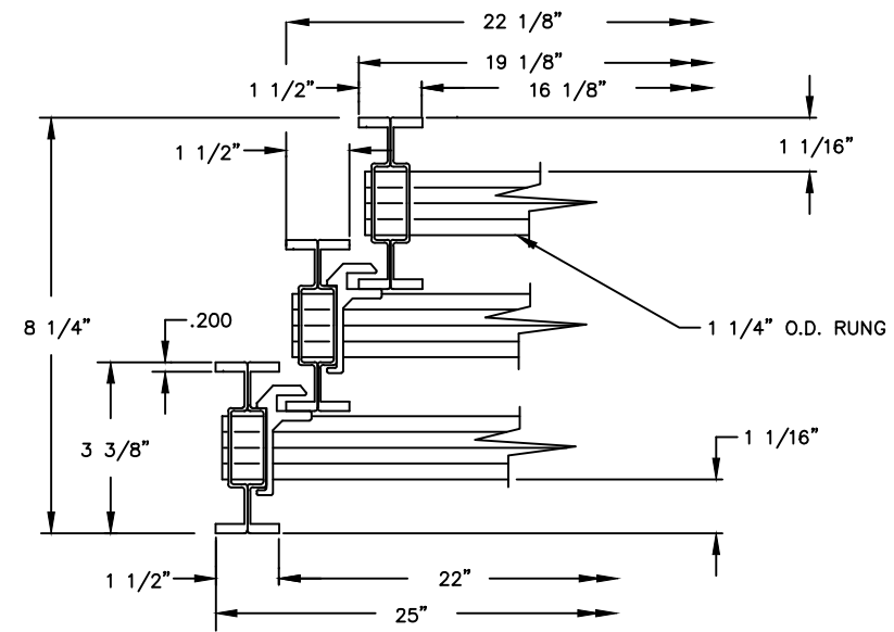
CROSS SECTION
